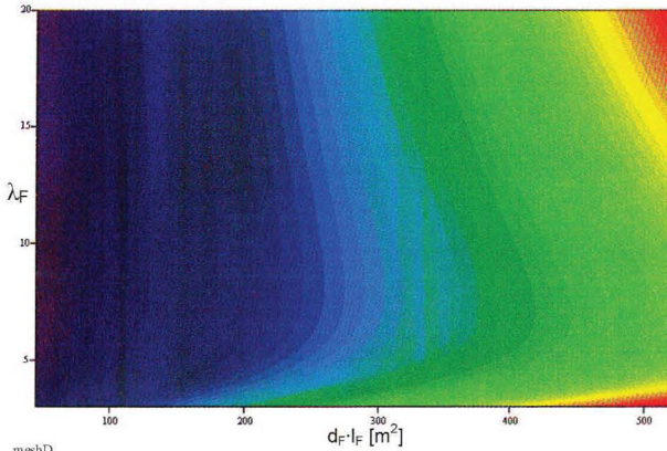
meshD FIG. 11 Total fuselage drag as a function of the slenderness and ( l_F \cdot d_F )
