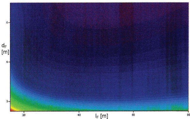
meshDv FIG. 10 Total drag of the fuselage-tail group relative to the volume ( d_F^2 \cdot l_F \cdot \pi/4 ) as a function of fuselage length and diameter
