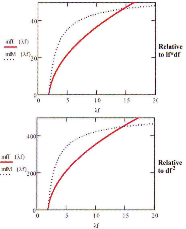
FIG. 21 Relative fuselage mass after Torenbeek (red) and Markwardt (blue) as a function of the slenderness parameter
