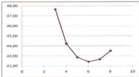
FIG. 23 Total drag of the fuselage-tail group relative to cabin surface ( I_F \cdot d_F ) as a function of number of seats abreast for a constant number of passengers
