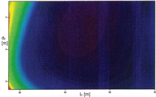
meshDes FIG. 8 Total drag of the fuselage-tail group relative to the cabin surface ( l_F \cdot d_F ) as a function of fuselage length and diameter
