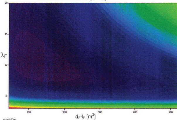
meshDes FIG. 12 Total fuselage drag relative to cabin surface ( l_F \cdot d_F ) as a function of the slenderness and ( l_F \cdot d_F )
