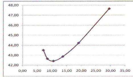
FIG. 25 Total drag of the fuselage-tail group relative to cabin surface ( I_F \cdot d_F ) as a function of the slenderness parameter for the selected values of the parameter n_{SA}
