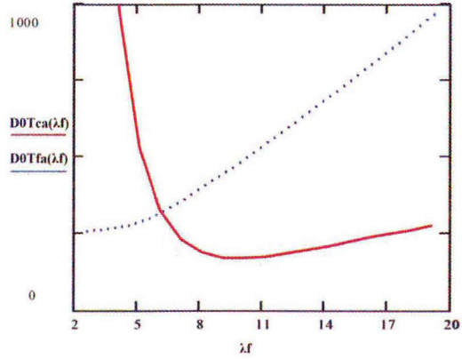
FIG. 17 Fuselage Zero Lift Drag as a function of slenderness: Cases 1.a, 1.b
