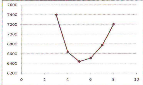
FIG. 22 Total drag of the fuselage-tail group as a function of number of seats abreast for a constant number of passengers
