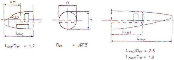
FIG. 7 Length of fuselage front and rear part [8]
