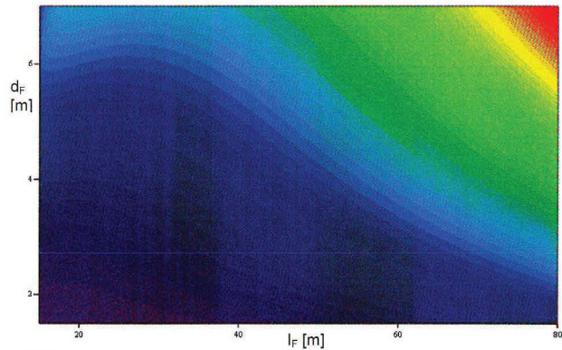
FIG. 7 Total drag of the fuselage-tail group as function of fuselage length and diameter
