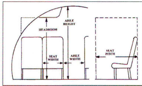
FIG. 3 Definition of important cabin and seat parameters [5]
