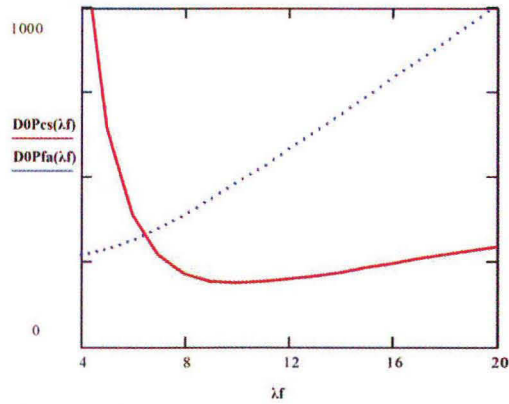
FIG. 18 Fuselage Zero Lift Drag as a function of slenderness: Cases 2.a, 2.b
