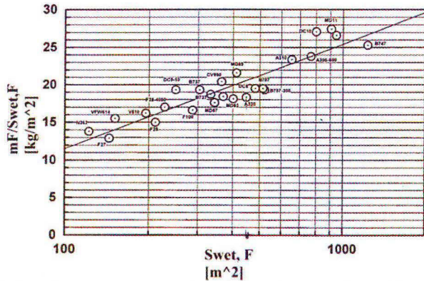
FIG. 20 m_F/S_{wet,F} as a function of the wetted area [7]
