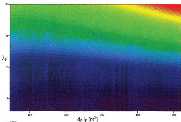
meshDü FIG. 13 Total fuselage drag relative to frontal area ( d_F^2 \cdot \pi/4 ) as a function of the slenderness and ( l_F \cdot d_F )
