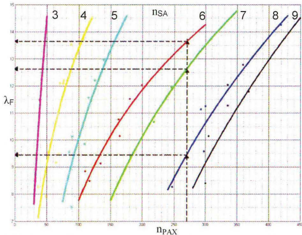
FIG. 2 Diagram showing the relation between the slenderness, number of passengers and number of seats abreast for 23 selected aircraft (magenta – n_{SA}=3 ; yellow – n_{SA}=4 ; light blue – n_{SA}=5 ; red – n_{SA}=6 ; green – n_{SA}=7 ; blue – n_{SA}=8 ; black – n_{SA}=9 )
