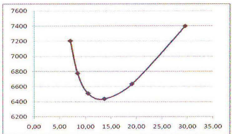
FIG. 24 Total drag of the fuselage-tail group as a function of slenderness for a constant number of passengers for the selected values of the parameter n_{SA}
