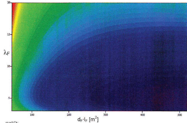
meshDv FIG. 14 Total fuselage drag relative to volume ( l_F \cdot d_F^2 \cdot \pi/4 ) as a function of the slenderness and ( l_F \cdot d_F )
