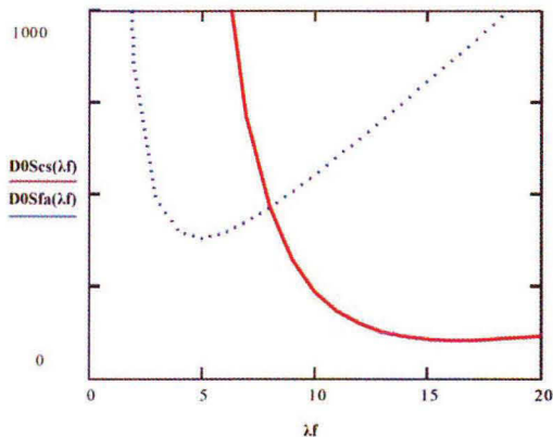
FIG. 19 Fuselage Zero Lift Drag as a function of fuselage slenderness: Cases 3.a, 3.b
