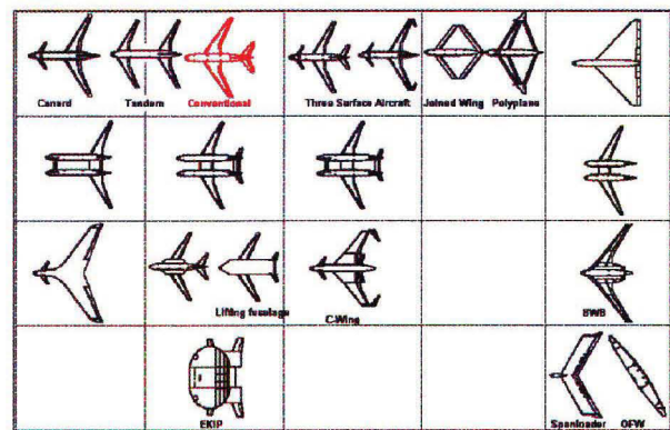
FIG.1 Wing and fuselage configuration concepts [1]
