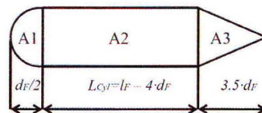
FIG. 15 Three parts approximation for the calculation of the wetted area
