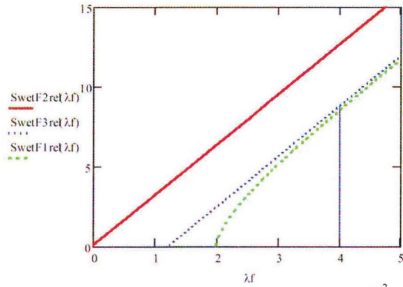
FIG. 16 Wetted area of the fuselage relative to d_F^2 as a function of the slenderness parameter: 1. Torenbeek (green), 2. Fuselage as a cylinder (red), 3. Fuselage as a sum of cockpit, tail and cabin (blue)
