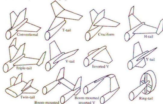
FIG. 6 Empennage configurations [5]
