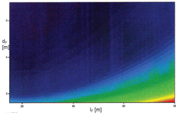
meshDiA FIG. 9 Total drag of the fuselage-tail group relative to the frontal area ( d_F^2 \cdot \pi/4 ) as a function of fuselage length and diameter
