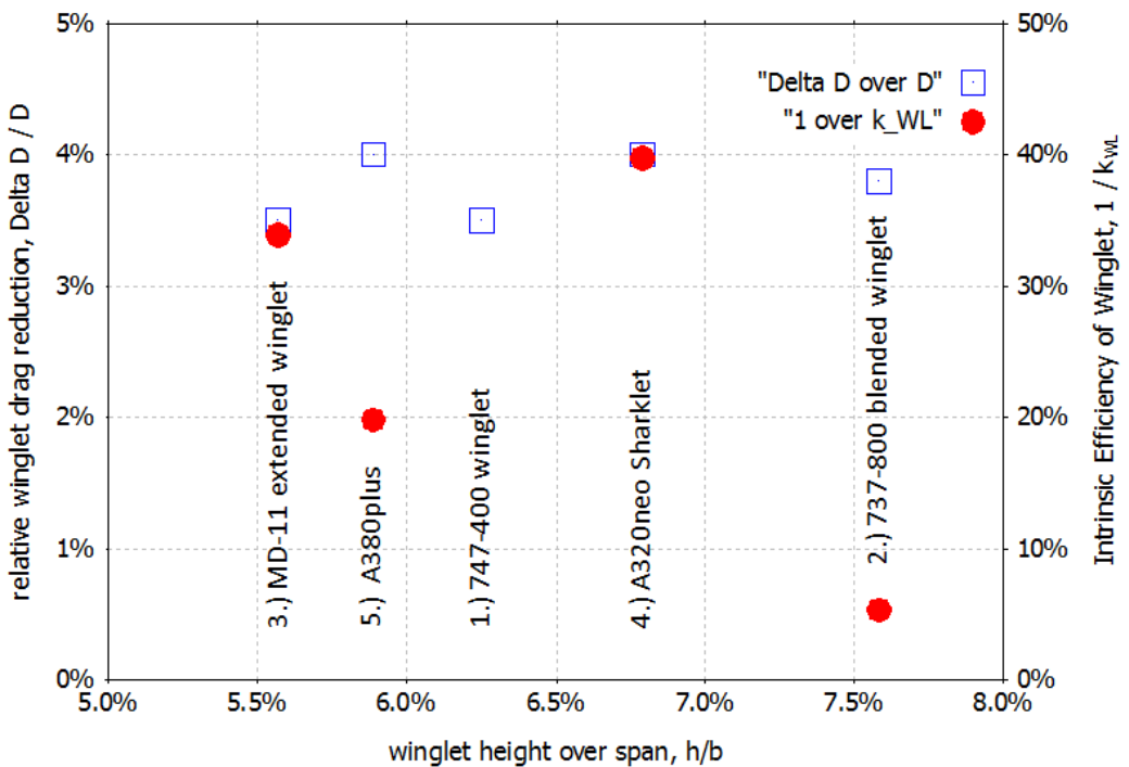
Fig. 8 – Relative drag reduction and Intrinsic Aerodynamic Efficiency of Winglets. Data from Table 2 and 3.
